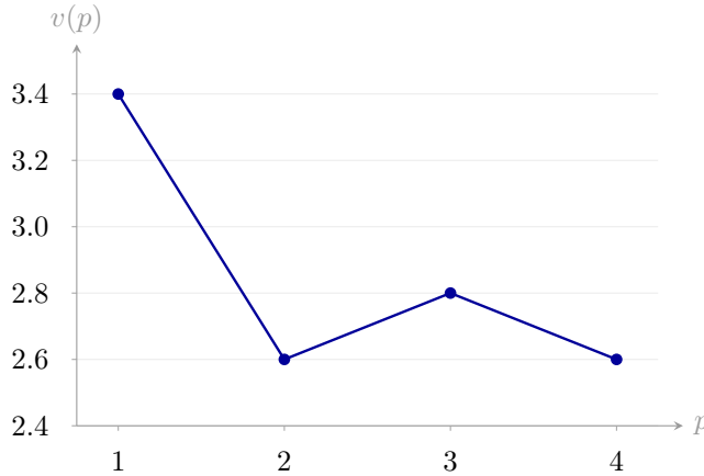
Figure 1: Optimal p -OBOP values for different numbers of buckets.
